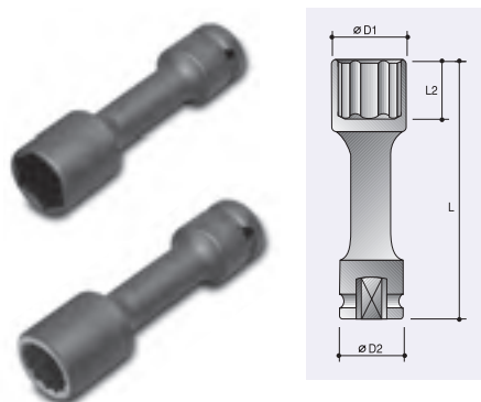
Wheel Nut Impact Socket
