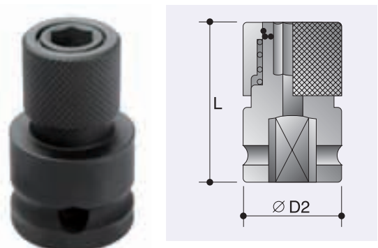
Quick Releasing Chucks
