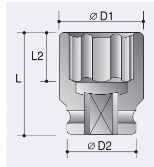
4-Point Sockets
