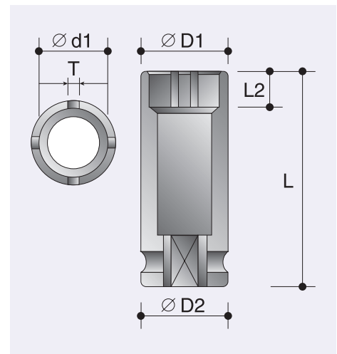
"KM" Type Axial Nut Sockets
