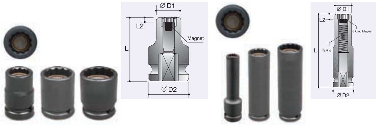
12-Point Sockets
