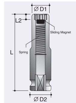
6-Point Sockets - Deep - With Slide Magnetic
