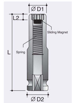
External Torx Sockets - Deep - With Slide Magnetic
