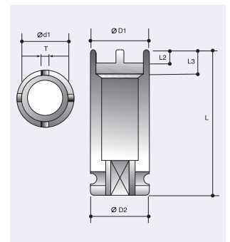
"GU" Type Axial Nut Sockets
