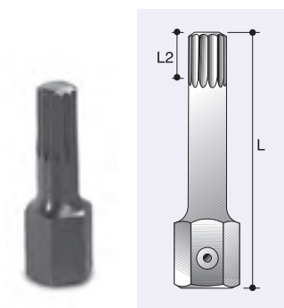
XZN - Triple Square
