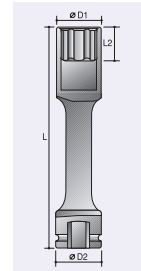
6-Point Extra Long Socket For Wheel Nuts
